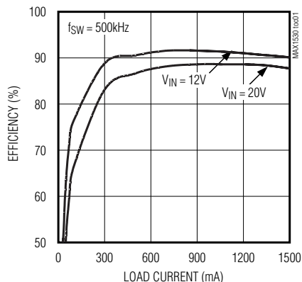
STEP-DOWN EFFICIENCY vs. LOAD CURRENT
