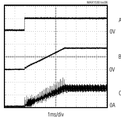
STEP-DOWN REGULATOR SOFT-START
