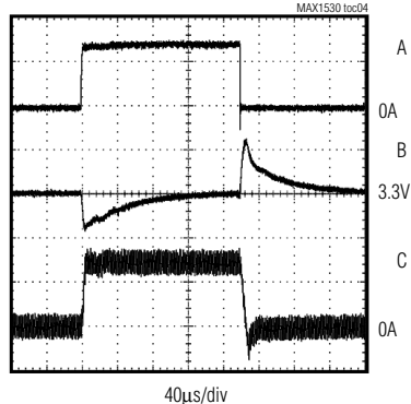
STEP-DOWN REGULATOR LOAD TRANSIENT
