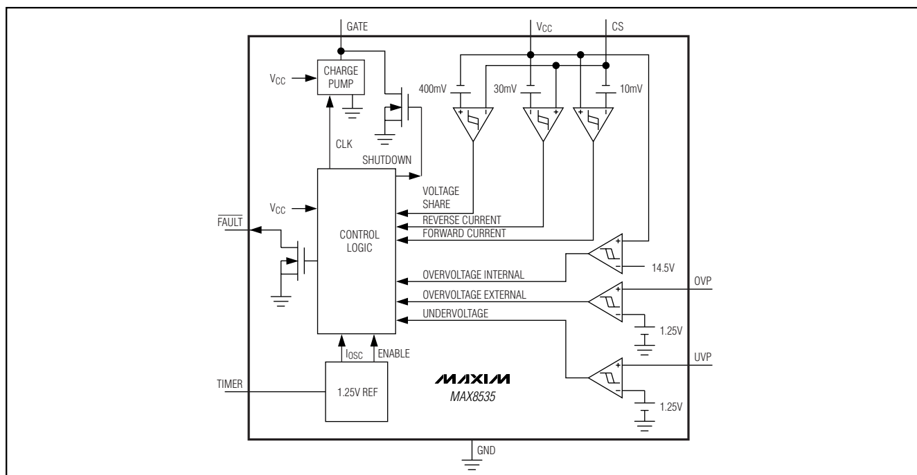
Figure 1. MAX8535 Functional Diagram
