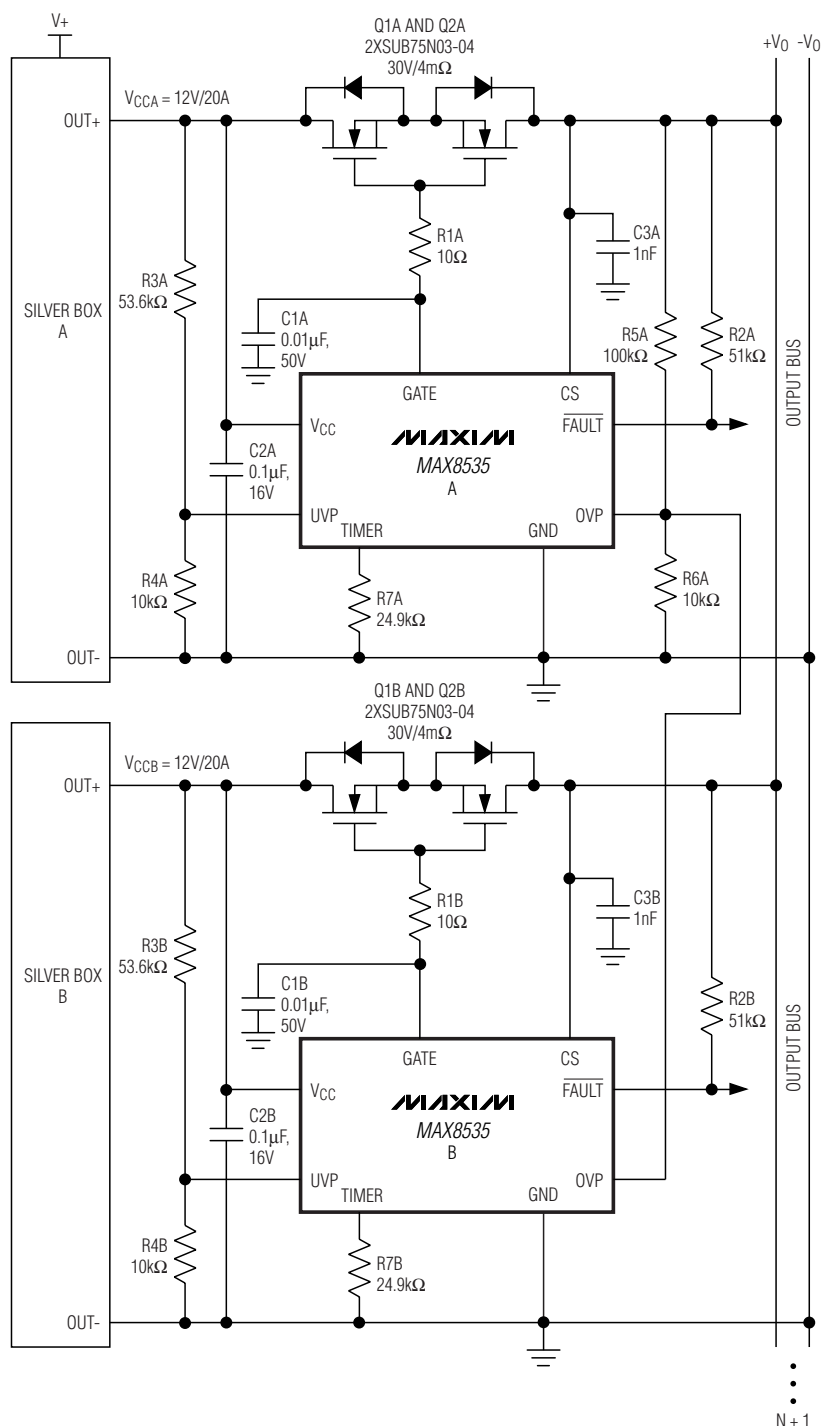
Figure 6. N + 1 Redundant Power System Connections
