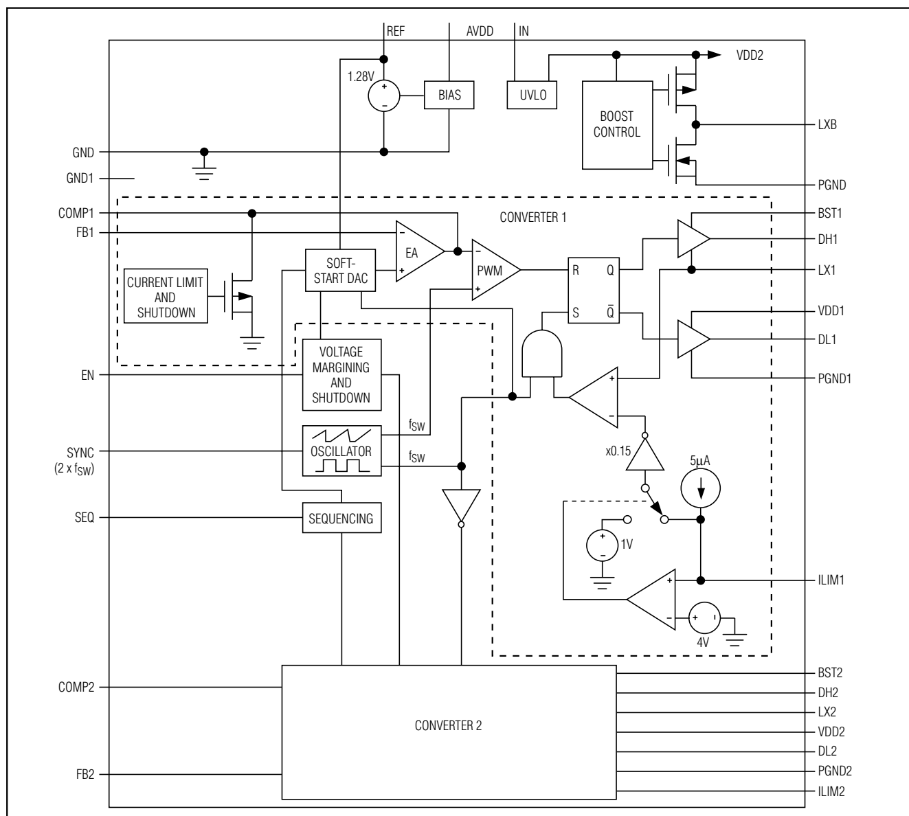
Figure 1. Functional Diagram
