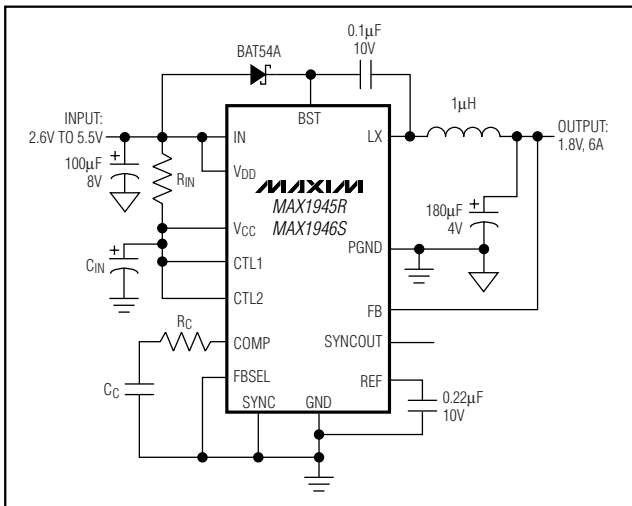
Figure 1. Typical Application Circuit (Fixed Output Voltage)
