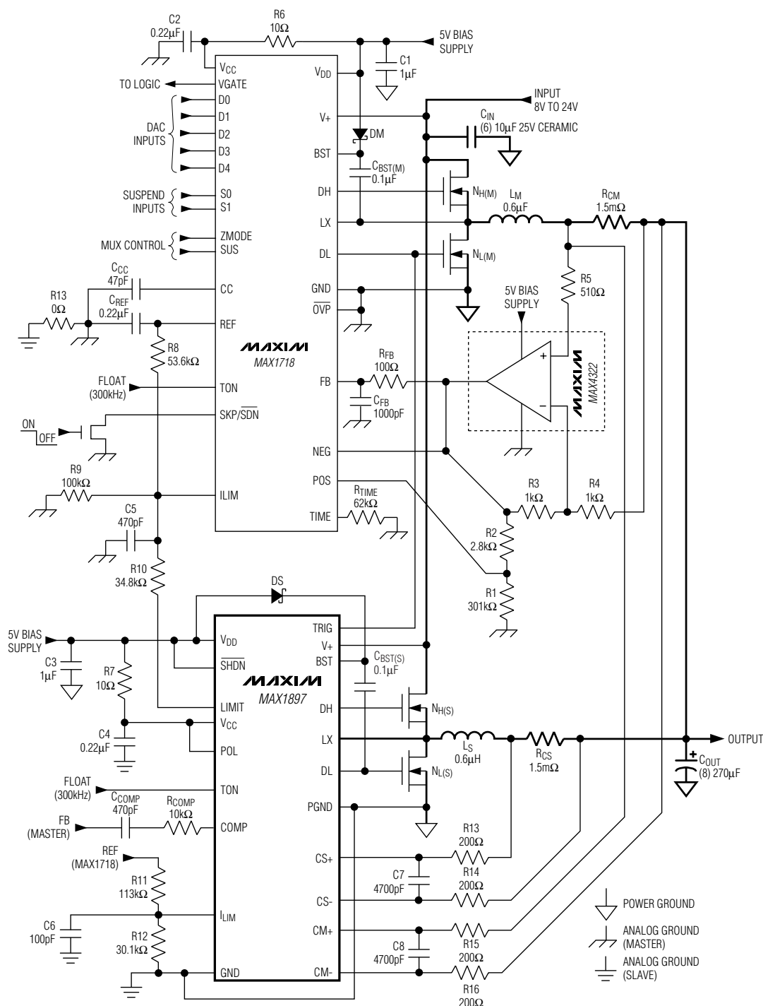
Figure 1. Standard Application Circuit
