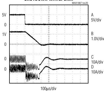
SHUTDOWN WAVEFORM
