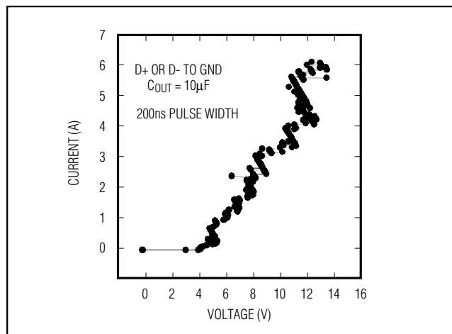
Figure 12. Transmission Line Pulsing I/V Characteristic (C OUT = 10 \mu F)
