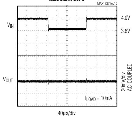
LINE-TRANSIENT RESPONSE REGULATOR 3
