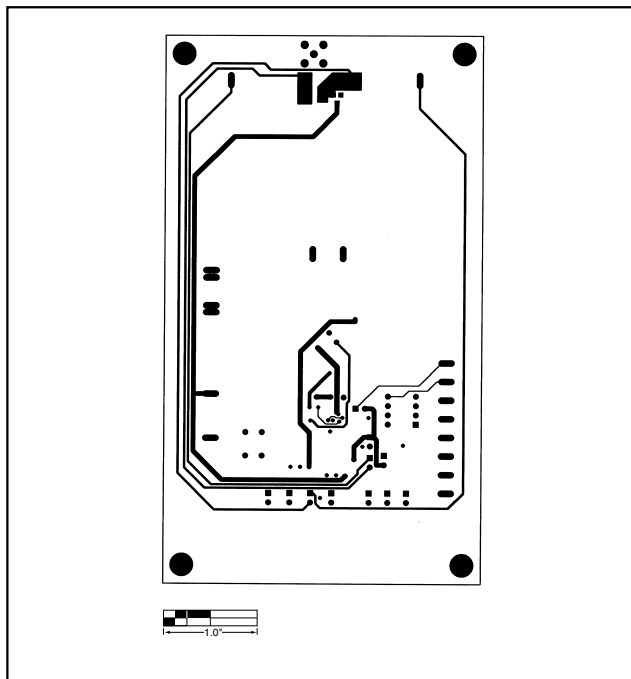
Figure 7. PC Board Layout—Solder Side
