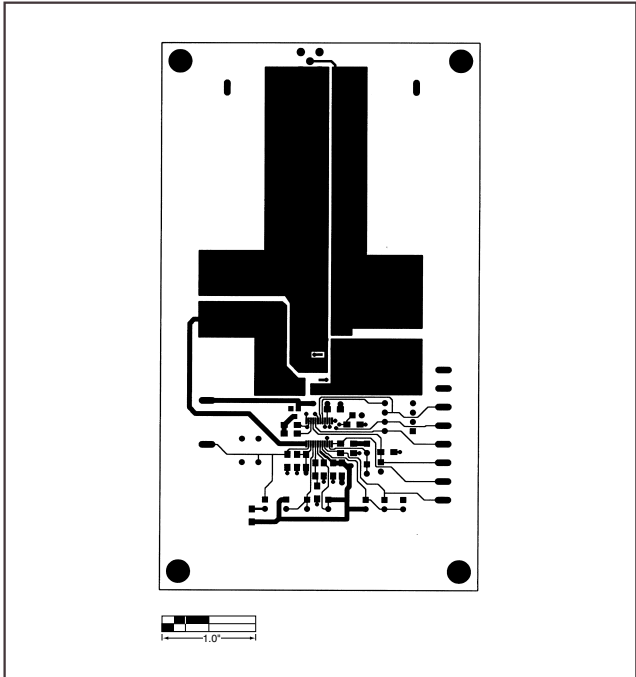
Figure 5. PC Board Layout—Component Side
