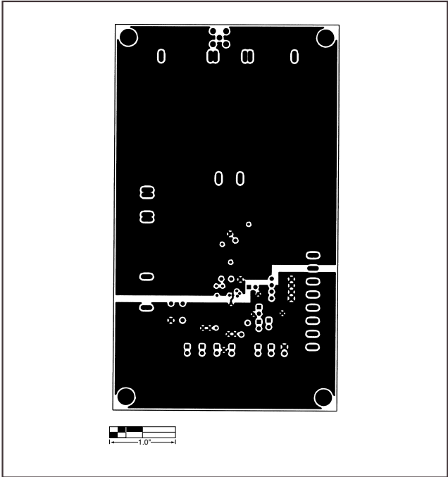
Figure 3. PC Board Layout—Internal GND Plane Layer 2
