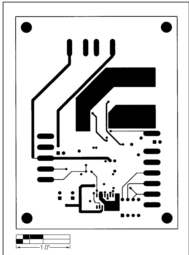
Figure 7. MAX1636 EV Kit PC Board Layout—Solder Side
