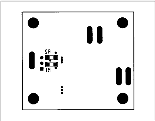
Figure 3. MAX764 EV Kit Component Placement Guide—Solder Side
