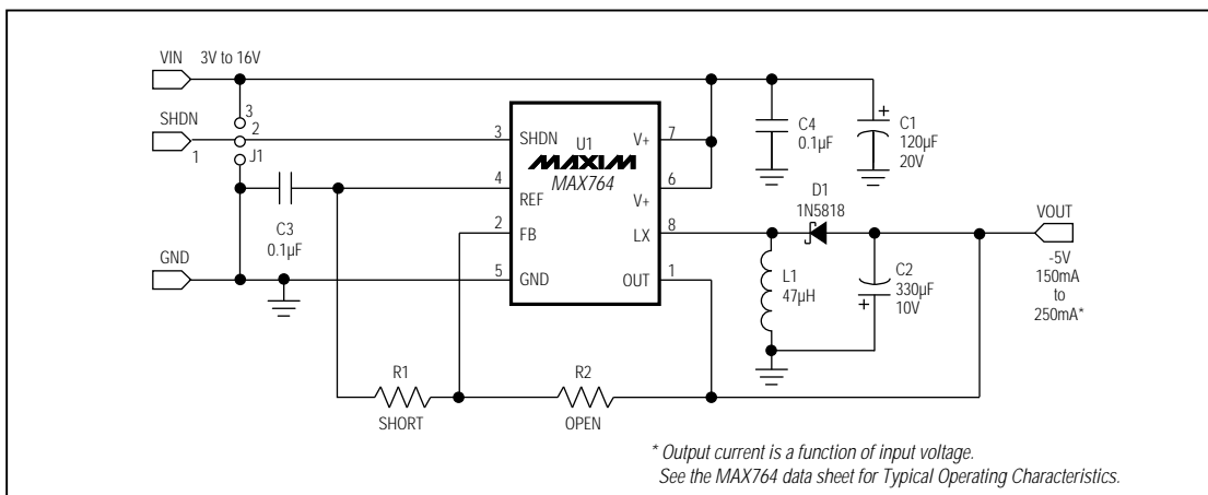
Figure 1. MAX764 EV Kit Schematic
