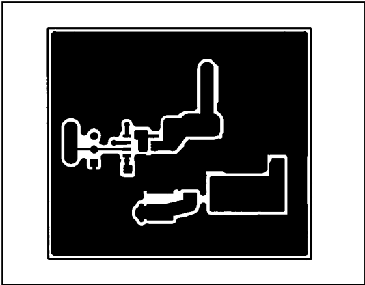
Figure 4. MAX764 EV Kit PC Board Layout—Component Side
