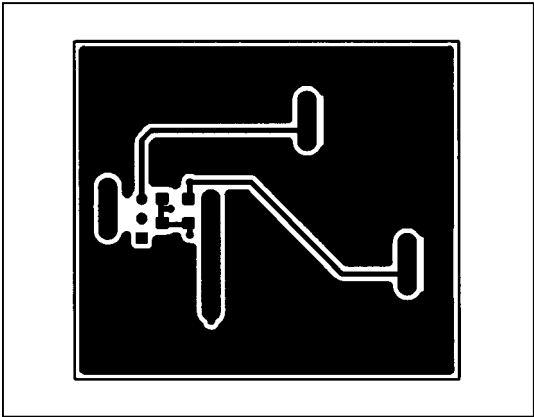
Figure 5. MAX764 EV Kit PC Board Layout—Solder Side
