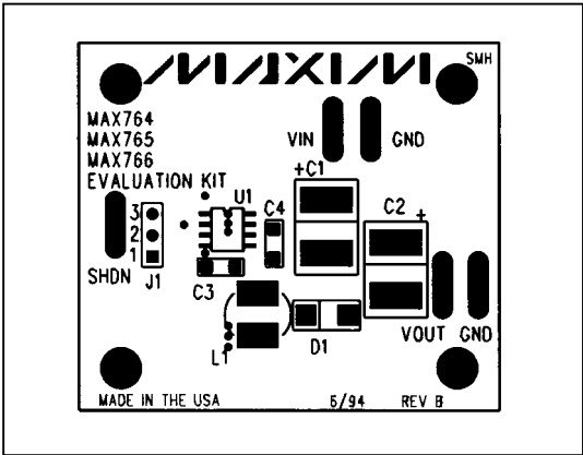
Figure 2. MAX764 EV Kit Component Placement Guide—Component Side
