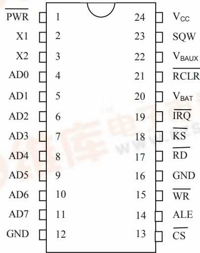
DS1685 24-Pin DIP
