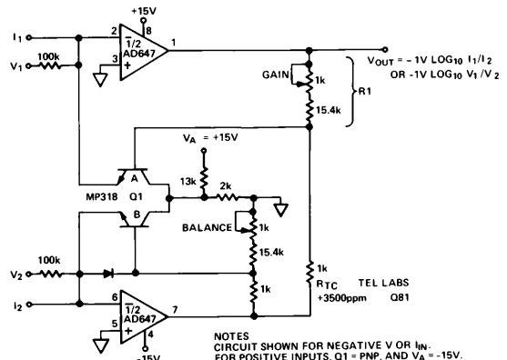
Figure 25. Log-Ratio Amplifier
