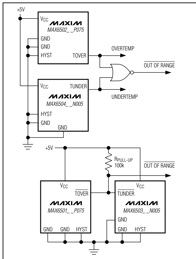
Figure 4. Temperature-Window Alarms
