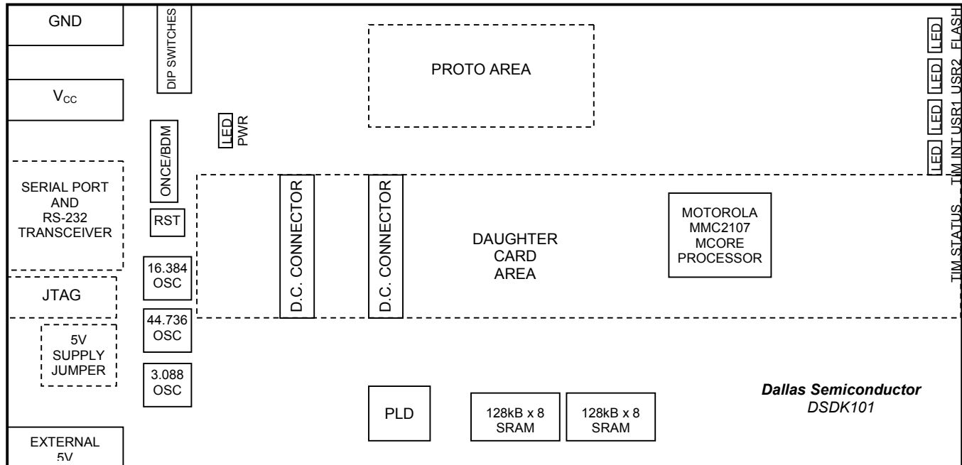
Figure 1. Board Floorplan
