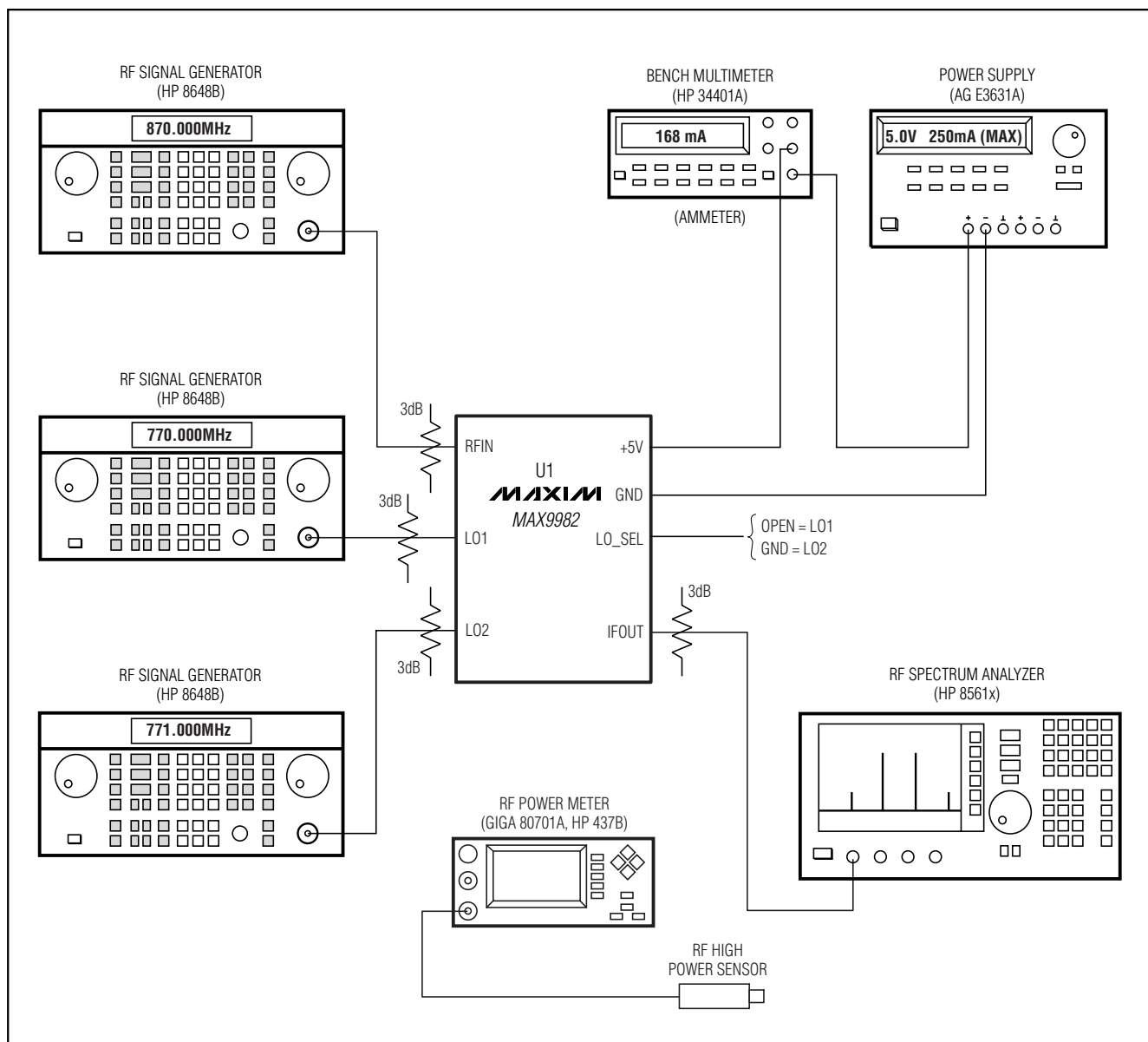
Figure 1. Test Setup Diagram
