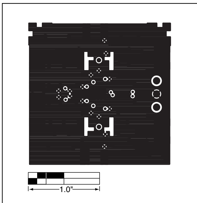
Figure 7. MAX9981 EV Kit PC Board Layout—Inner Layer 2 (GND)
