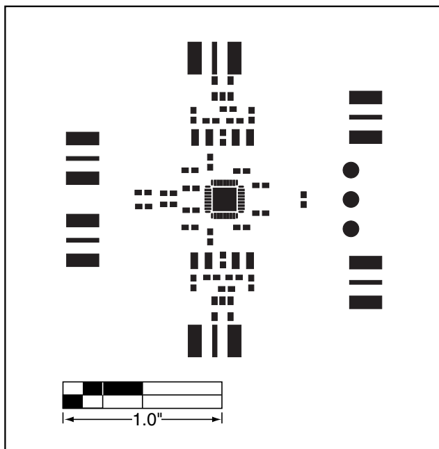
Figure 5. MAX9981 EV Kit PC Board Layout—Top Soldermask
