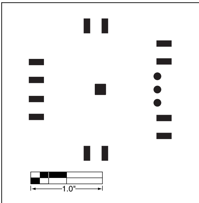
Figure 10. MAX9981 EV Kit PC Board Layout—Bottom Soldermask
