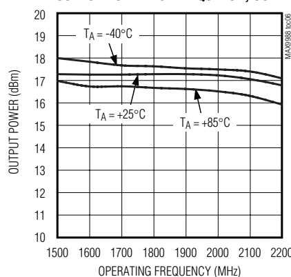
OUTPUT POWER vs. FREQUENCY, OUT2
