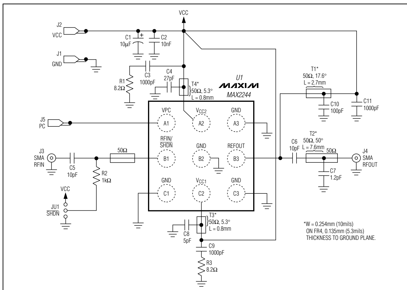
Figure 1. MAX2244 EV Kit Schematic
