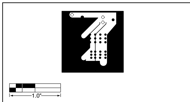
Figure 6. MAX2244 EV Kit PC Board Layout—Power Plane
