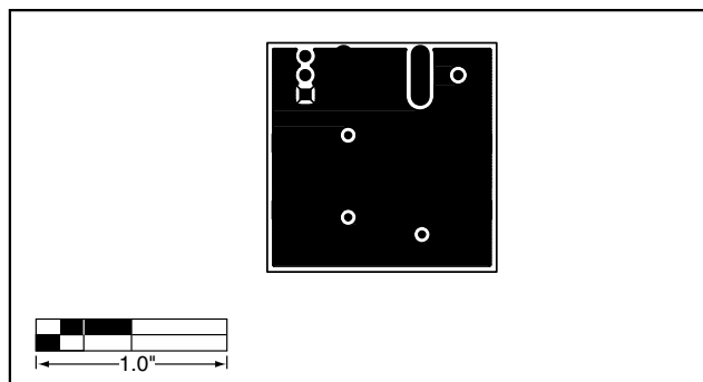
Figure 7. MAX2244 EV Kit PC Board Layout—Solder Side
