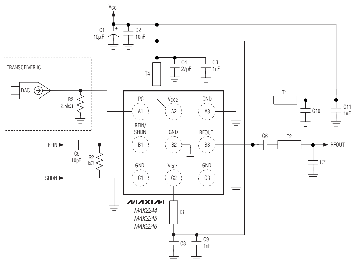
Figure 1. MAX2244/MAX2245/MAX2246 Typical Application Circuit
