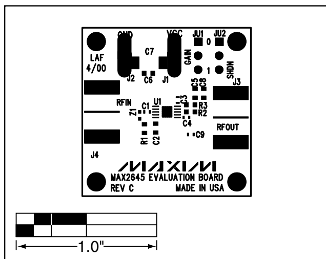
Figure 2. MAX2645 EV Kit PC Board Layout—Component Placement Guide
