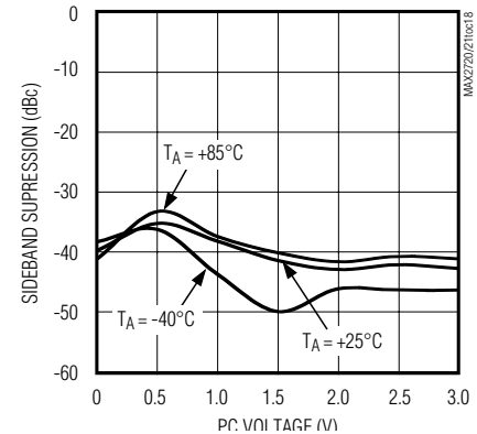
MODULATOR SIDEBAND SUPPRESSION vs. PC VOLTAGE (ENX2 = VCC)
