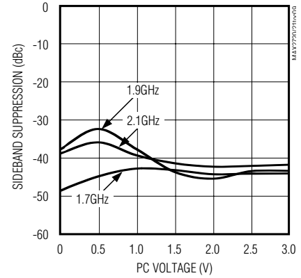
MODULATION SIDEBAND SUPPRESSION vs. PC VOLTAGE (ENX2 = GND)
