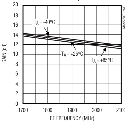
PA DRIVER GAIN vs. RF FREQUENCY
