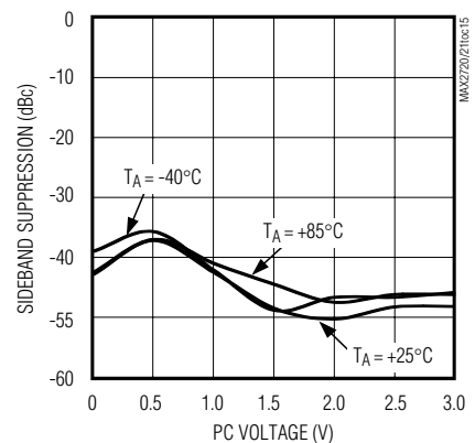
MODULATOR SIDEBAND SUPPRESSION vs. PC VOLTAGE (ENX2 = GND)
