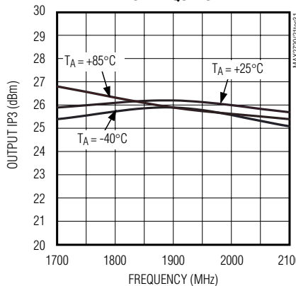
PA DRIVER OUTPUT IP3 vs. FREQUENCY
