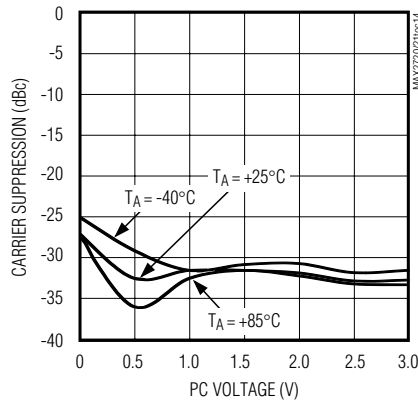
MODULATOR CARRIER SUPPRESSION vs. PC VOLTAGE (ENX2 = GND)
