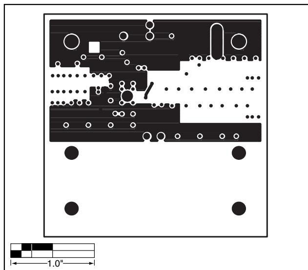
Figure 5. MAX2235 EV Kit PC Board Layout—Power Plane
