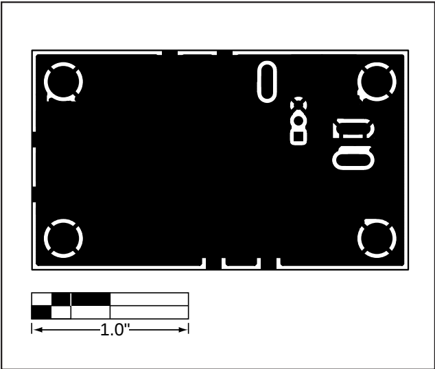
Figure 4. MAX2680/MAX2681/MAX2682 EV Kits PC Board Layout —Ground Plane
