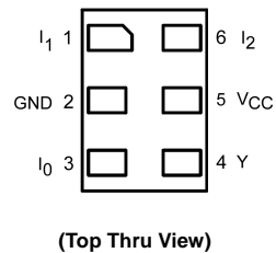
Pad Assignments for MicroPak
