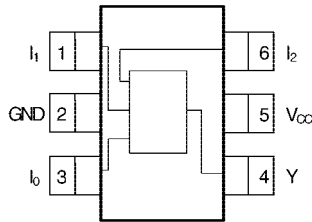
(Top View) NC7SP57 and NC7SP58
