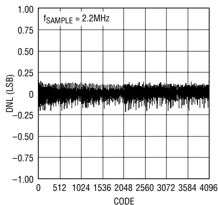
Differential Nonlinearity vs Output Code (Bipolar)
