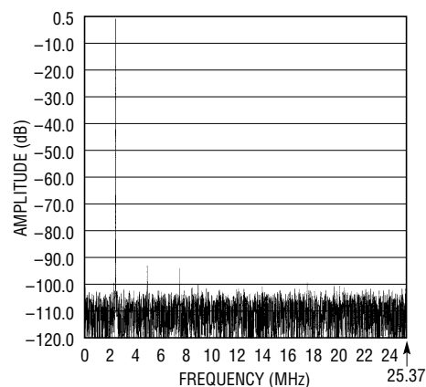
Nonaveraged, 8192 Point FFT, Input Frequency = 2.5MHz, 2V Range
