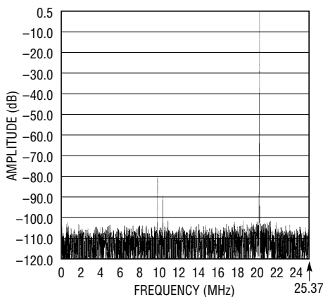
Nonaveraged, 8192 Point FFT, Input Frequency = 20MHz, 3.2V Range
