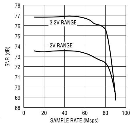
SNR vs Sample Rate, Input Frequency = 5MHz
