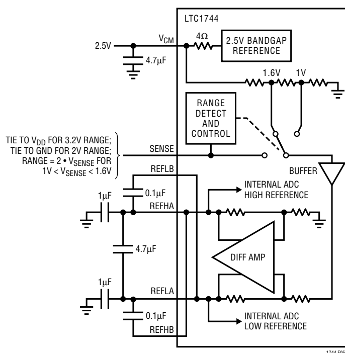
Figure 5. Reference Circuit
