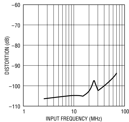
Worst Harmonic 4th or Higher vs Input Frequency, 2V Range
