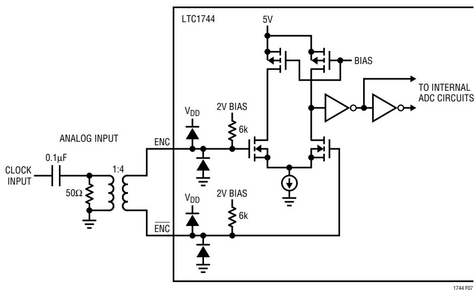
Figure 7. Transformer Driven ENC/ENC-bar
