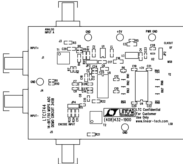
Topside Silkscreen
