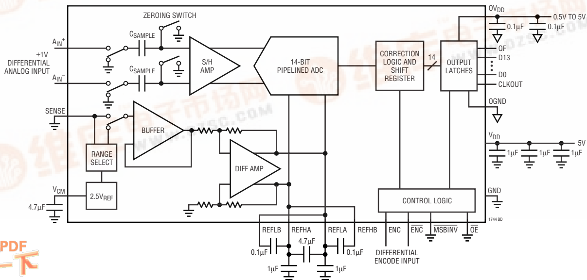
50Msps, 14-Bit ADC with a \pm 1V Differential Input Range
