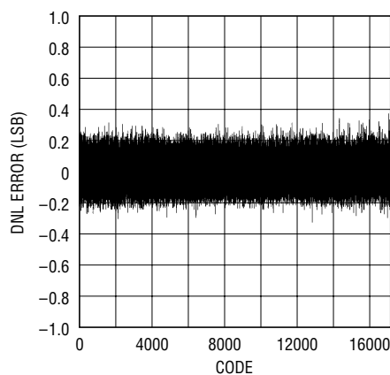
Typical DNL
