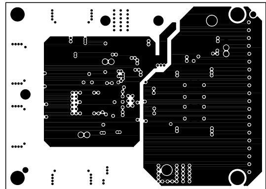
Split Power Plane, Layer 3
