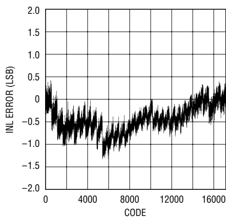
Typical INL
