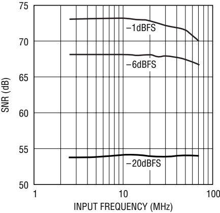
SNR vs Input Frequency, 2V Range
