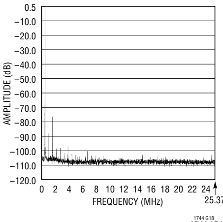
Averaged, 8192 Point FFT, Input Frequency = 51MHz, -1dB, 2V Range
