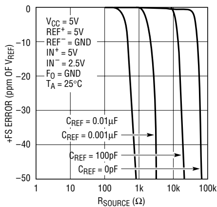
Figure 25. +FS Error vs R_{SOURCE} at REF + or REF - (Small C_{REF} )
