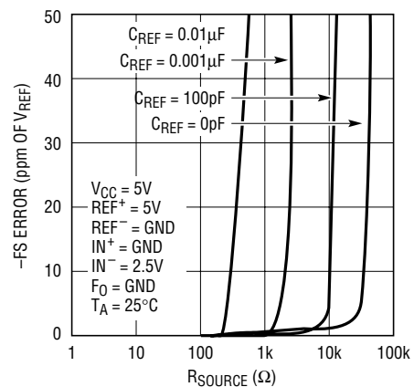
Figure 26. -FS Error vs R_{SOURCE} at REF + or REF - (Small C_{REF} )
