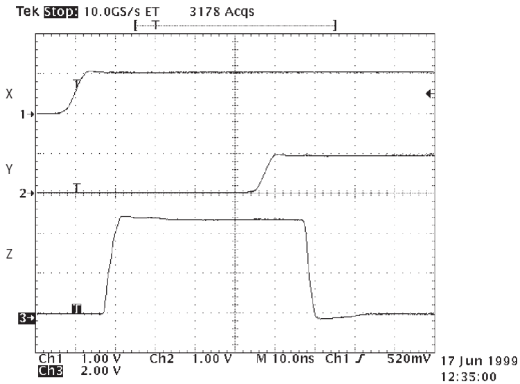
Figure 13. Output Pulse Due to Delay of Input Pulse
