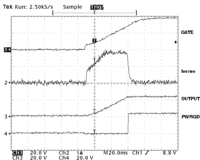
Figure 6. Power-Up Waveforms
