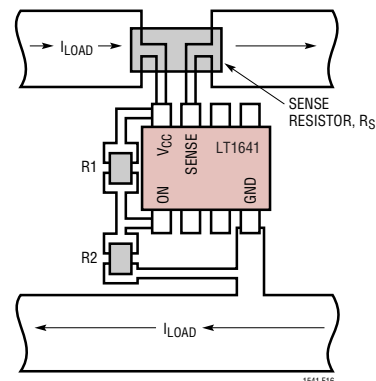
Figure 16. Recommended Layout for R1, R2 and R_S
