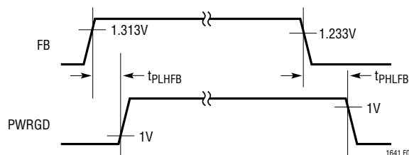
Figure 3. FB to PWRGD Timing
