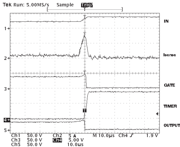
Figure 13. Overvoltage Waveforms
