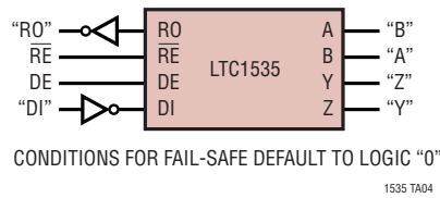
Figure 19. Fail-Safe Logic "0"
