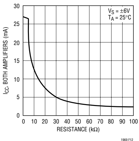
Figure 12. Supply Current vs Control Resistance (R1//R2)
