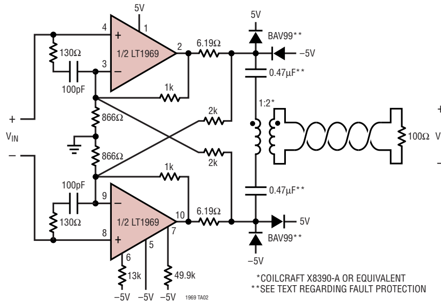
Split Supply \pm 5V ADSL CPE Line Driver
