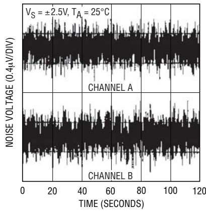
0.01Hz to 10Hz Noise
