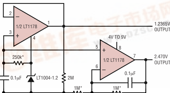
Self-Buffered, Dual Output, Micropower Reference
