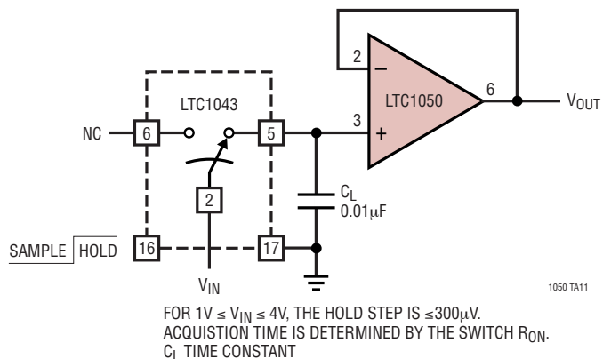
Sample-and-Hold Amplifier
