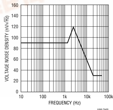
Noise Spectrum
