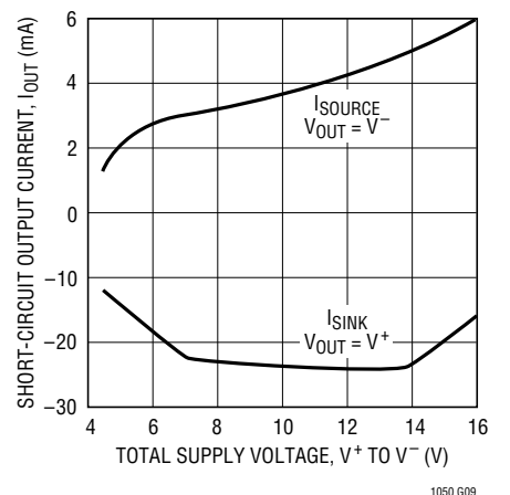
Short-Circuit Output Current vs Supply Voltage
