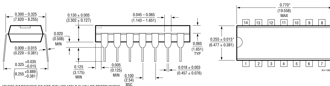
N Package 14-Lead PDIP (Narrow .300 Inch) (Reference LTC DWG # 05-08-1510)
