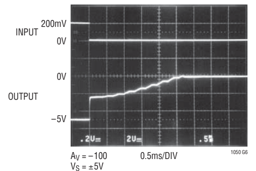
Overload Recovery
