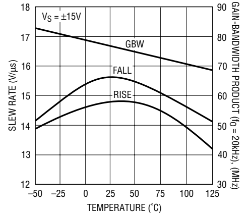
LT1028 Slew Rate, Gain-Bandwidth Product Over Temperature
