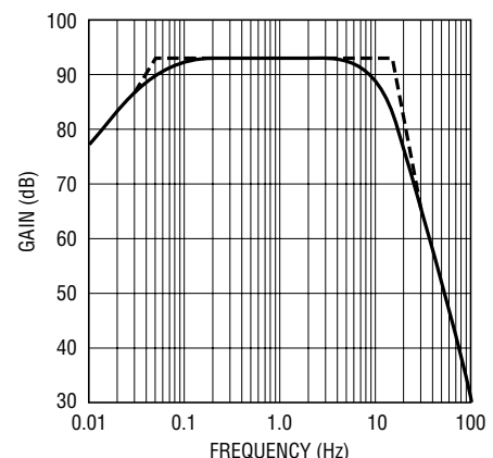
0.1Hz to 10Hz Peak-to-Peak Noise Tester Frequency Response
