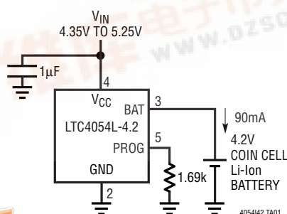
90mA Li-Ion Single Coin Cell Charger
