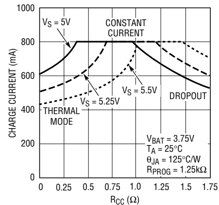
Figure 3. Charge Current vs R_{CC}
