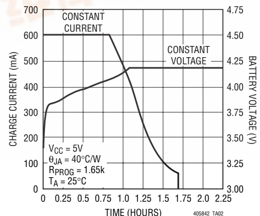
Complete Charge Cycle (750mAh Battery)
