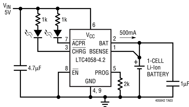
Full Featured Single Cell Li-Ion Charger
