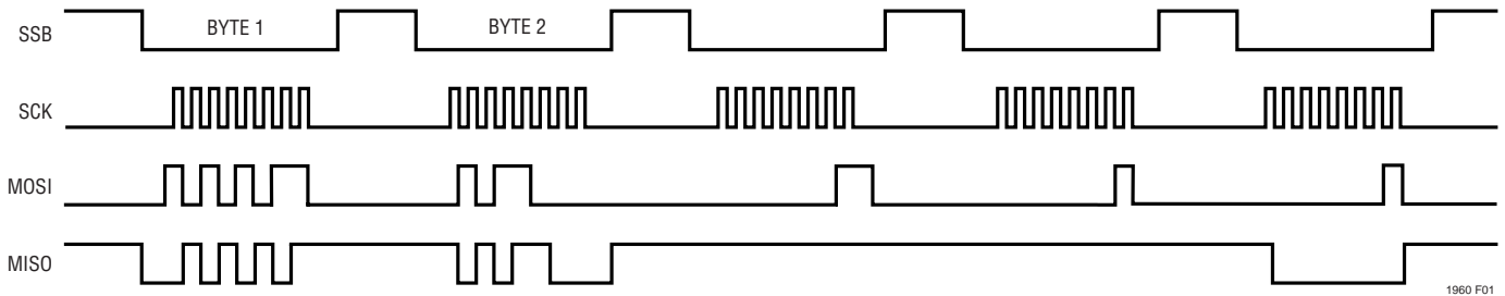
Figure 1. SPI Write to VDAC of Data = b101_0101_0101
