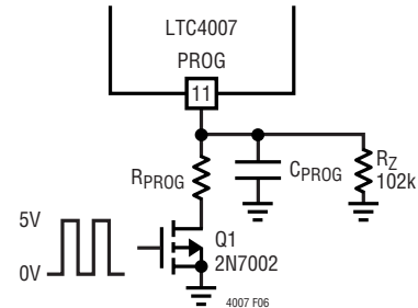
Figure 6. PWM Current Programming
