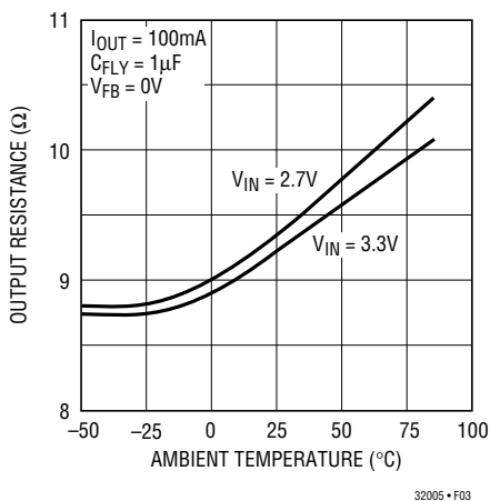
Figure 3. Typical R_{OL} vs Temperature
