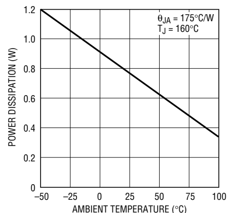
Figure 6. Maximum Power Dissipation vs Ambient Temperature
