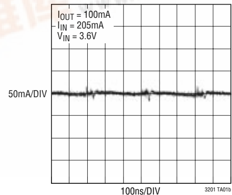
Input Current Ripple
