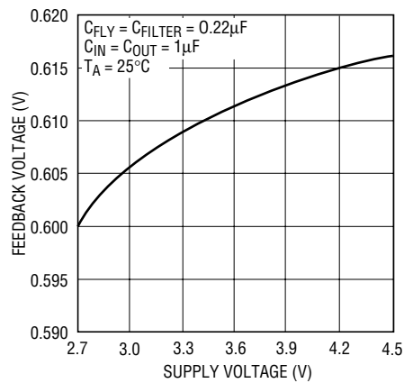
Feedback Voltage vs Supply Voltage I_{OUT} = 100\text{mA} , V_{OUT} = 4\text{V}
