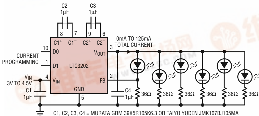
Programmable White LED Power Supply
