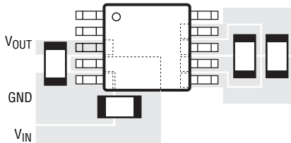
Figure 6. Recommended Layout
