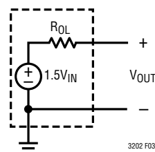
Figure 3. Equivalent Open-Loop Circuit
