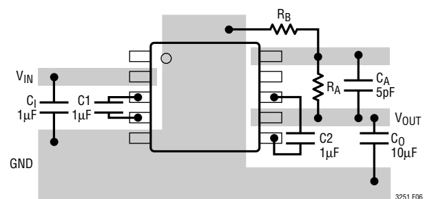
Figure 6. Recommended Layout
