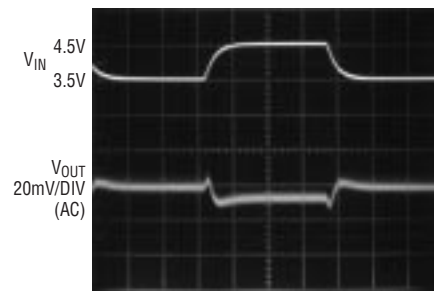
Supply Transient Response (Continuous Mode)
