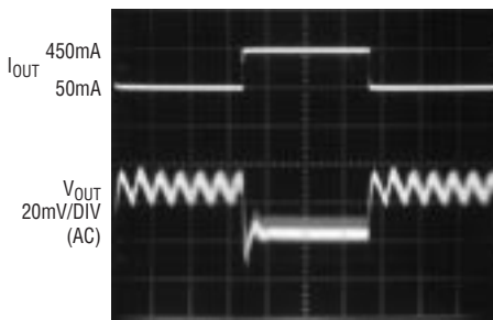
Output Transient Response (Burst Mode Operation)
