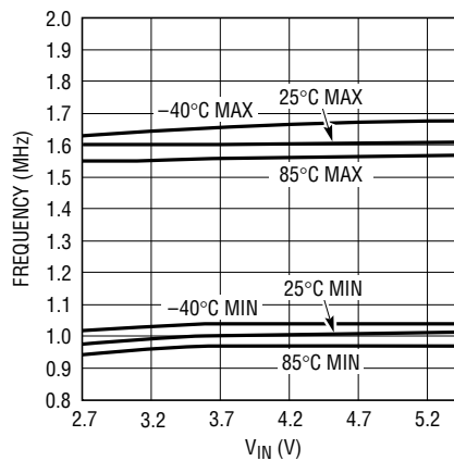
Max/Min Oscillator Frequency vs Supply Voltage
