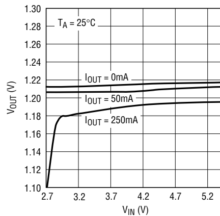
1.2V Output Voltage vs Supply Voltage
