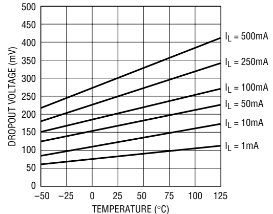
Dropout Voltage
