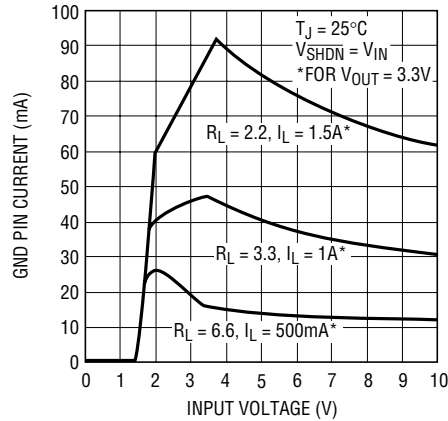
LT1963A-3.3V GND Pin Current
