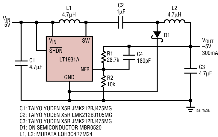
2.2MHz, 5V to -5V Inverting Converter
