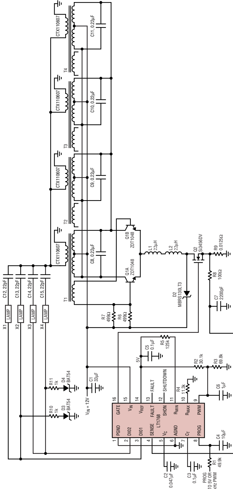
24 Watt Four Lamp CCFL Supply
