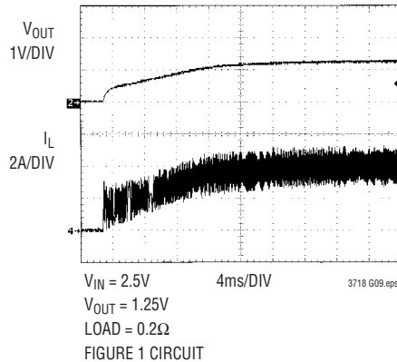
Start-Up Response
