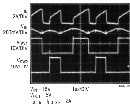
Input Source/Capacitor Instantaneous Current (Figure 1)
